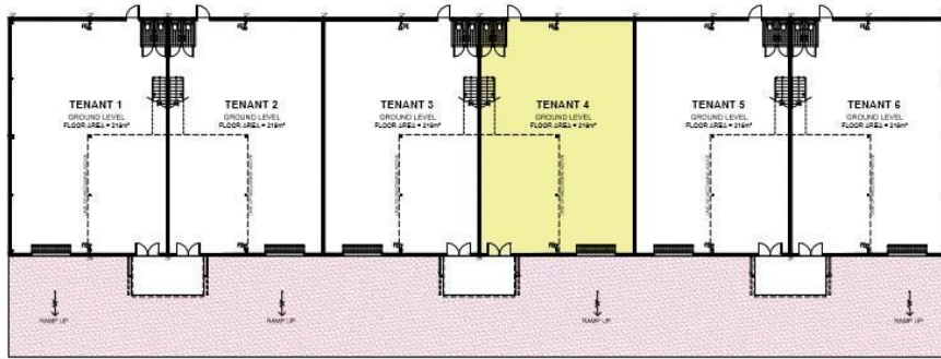
ELEVATION KEY GROUND FLOOR PLAN SCALE A3 @ 1:200 A1 @ 1:100
